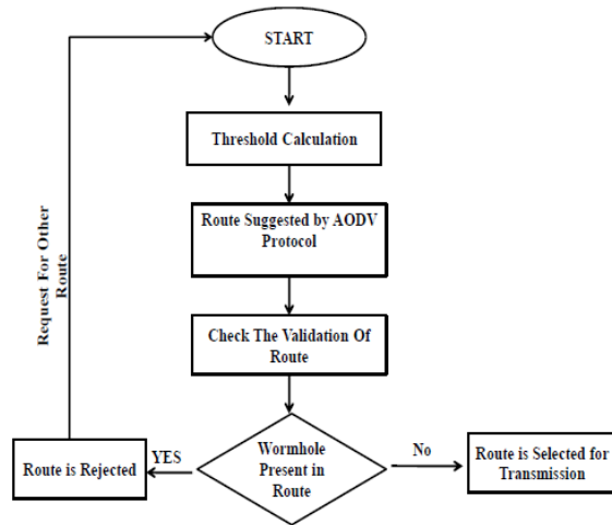
Figure 1: Flow Chart of Proposed Algorithm
